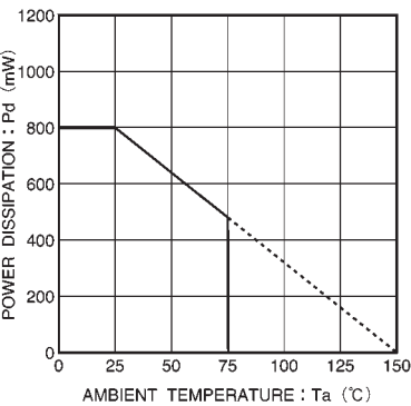
Fig.6 Power dissipation curve
